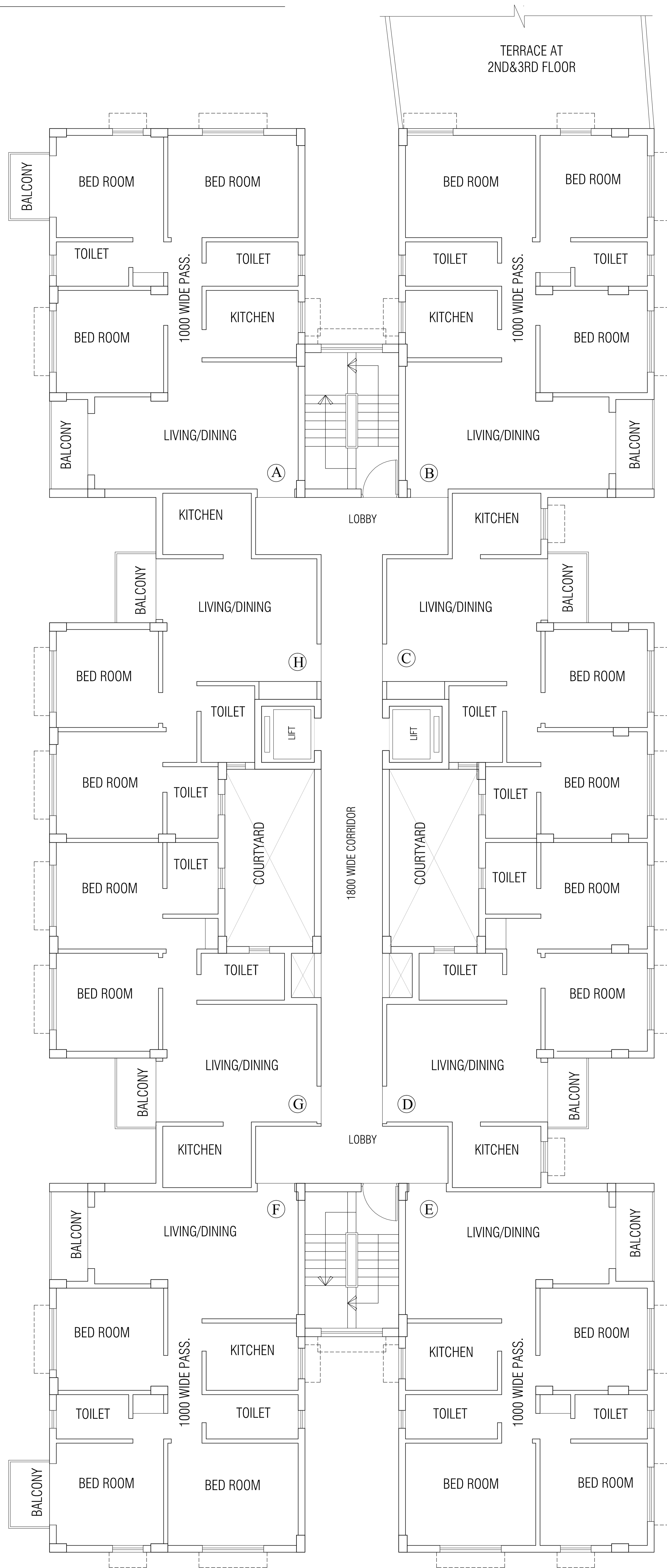
TYPICAL FLOOR PLAN (BLOCK - 3) SCALE - NTS
